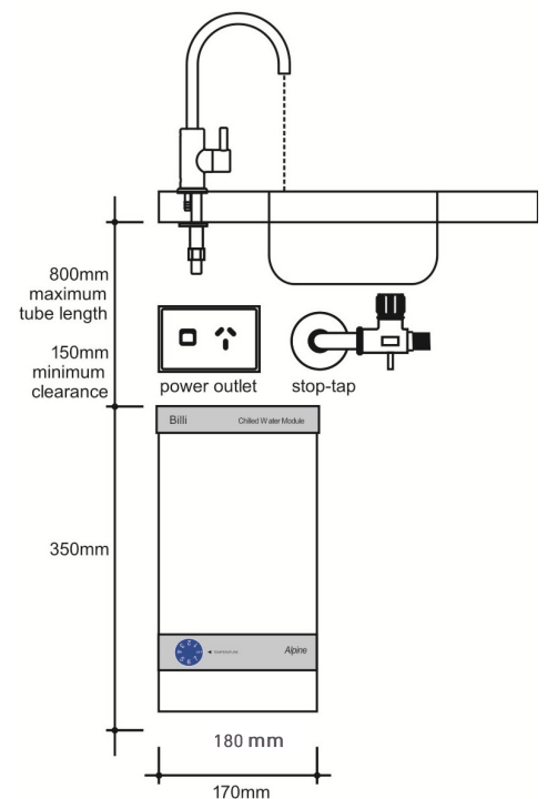
Preferred installation layout
