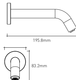
Billi KwikWash Wall Mount Sensor Tap dimensions
