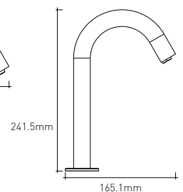
Billi KwikWash Bench Mount Sensor Tap dimensions
