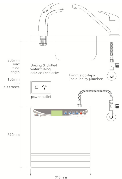
Preferred installation layout
