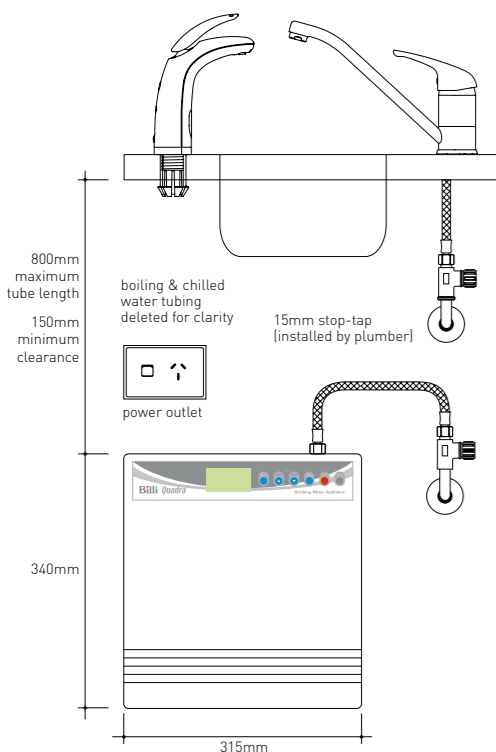
Preferred installation layout Minimum cupboard dimensions: Water-cooled unit: 475mm depth x 335mm width Air-cooled unit: 520mm depth x 365mm width
