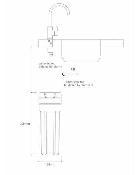
Preferred installation layout
