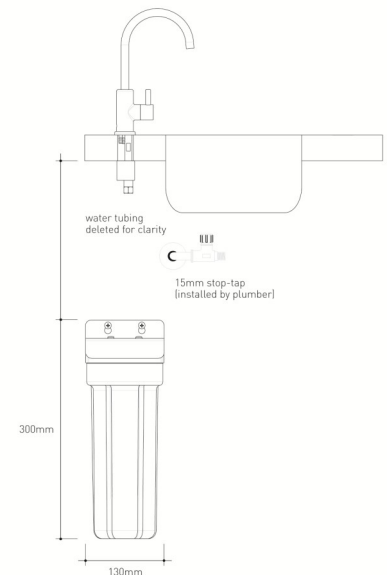
Preferred installation layout
