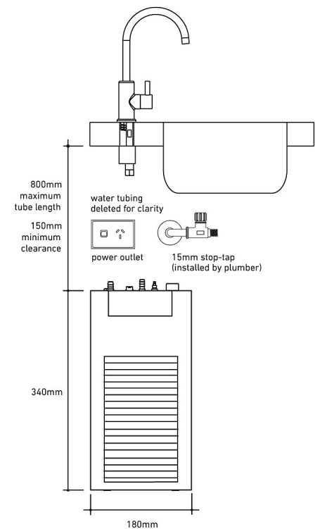
Preferred installation layout
