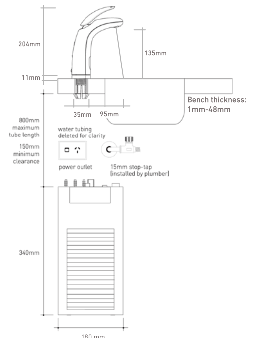
Preferred installation layout
