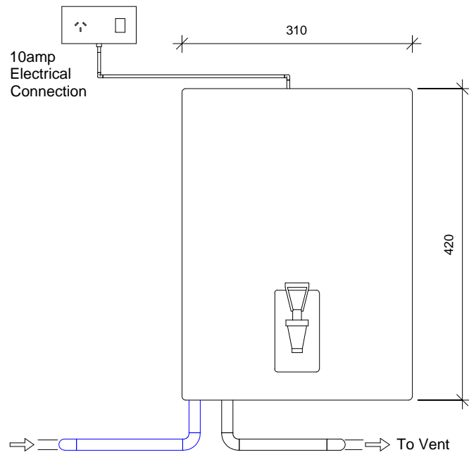
Billi Ultra Front View
